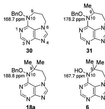
FIGURE 2. Examples of the \beta -effect in 15 N NMR on N-10 by the 9-substituents.
