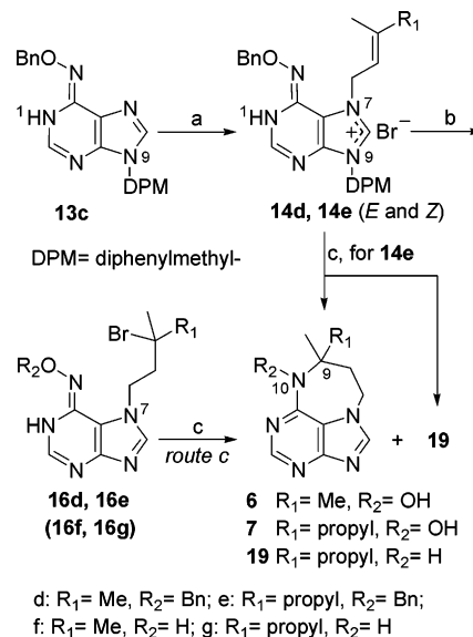
SCHEME 3. Route c Leading to 9,9-Disubstituted 10-Hydroxy-THDAP a
