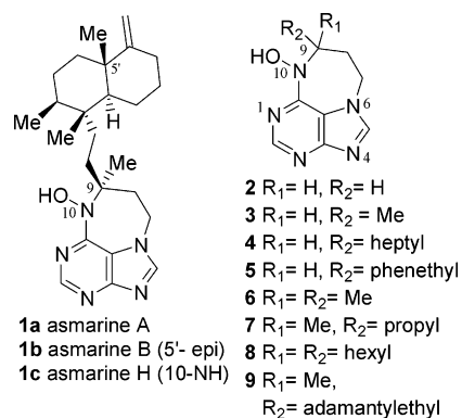
FIGURE 1. Asmarines 1a–c and synthetic analogues 2–9 .
